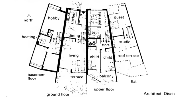
6 Terraced houses orientated for favourable lighting and sunshine
